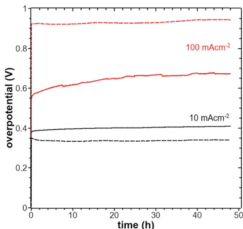
Fig. 38 Plot of the overpotential as a function of time at current densities of 10 \text{ mA cm}^{-2} (black) and 100 \text{ mA cm}^{-2} (red) measured in 1 M KOH for films deposited at 50 \text{ }^{\circ}\text{C} (dashed lines) and 103 \text{ }^{\circ}\text{C} (full lines). Reproduced with permission from ref. 733. Copyright American Chemical Society 2020.
