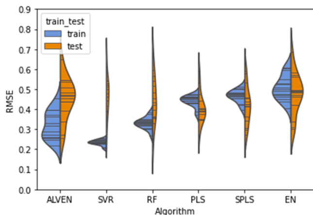
Fig. 5. Model prediction results for mAb#1 data with logarithm of output.
