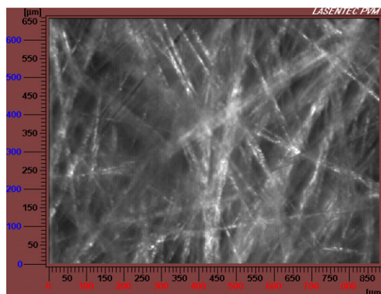
Fig. 16. PVM image of lovastatin crystals.
