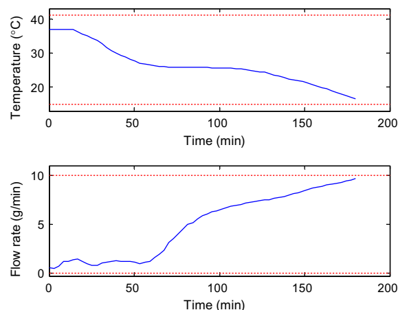
Fig. 9. Optimal operating curves for the combined crystallization with objective J_{n,m.s.}
