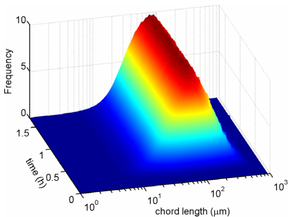
Fig. 13. FBRM CLD for the antisolvent system.
