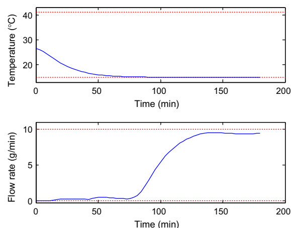
Fig. 10. Optimal operating curves for the combined crystallization with objective J_{n,s,r}
