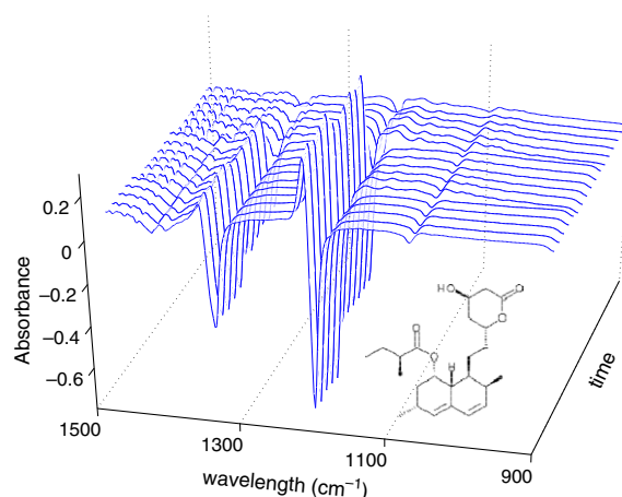
Fig. 3. Molecular formula and IR spectra of lovastatin at different temperatures, concentrations, and solvent/antisolvent ratios.
