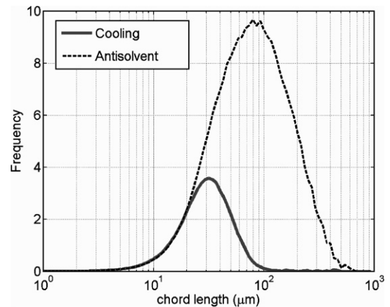
Fig. 15. CLD at the end of the batch for the cooling and antisolvent systems.
