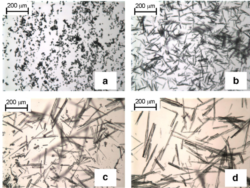
Fig. 11. Microscopic images of seed (a) and product crystals for the three operating modes: (b) cooling-only, (c) antisolvent-only, and (d) combined.
