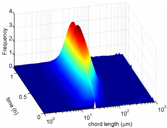
Fig. 12. FBRM CLD for the cooling-only system.
