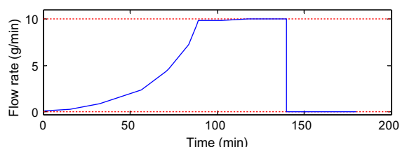
Fig. 8. Optimal flowrate profile for antisolvent crystallization with objective J_{n,m.s.}
