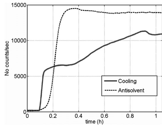
Fig. 14. Total number of counts from FBRM.
