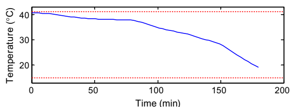
Fig. 7. Optimal temperature profile for cooling crystallization with objective J_{n,m.s.}
