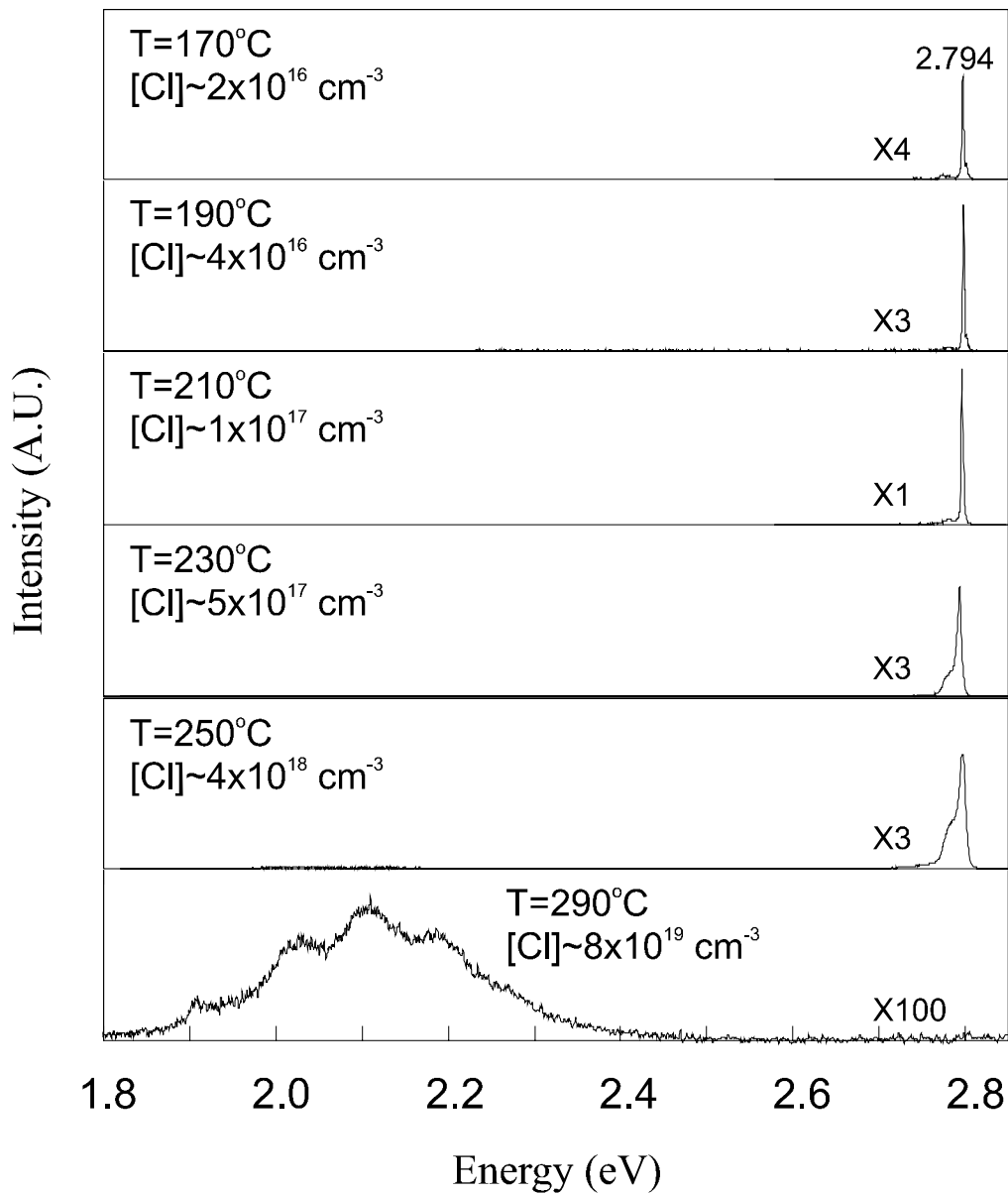
Figure 3-7 10K photoluminescence of Cl-doped ZnSe films having a progressively higher doping concentration from the top to the bottom subplots. The \text{ZnCl}_2 cell temperature, relative magnifications used to obtain the spectrum, as well as the [\text{Cl}] determined by SIMS are indicated in each case.
