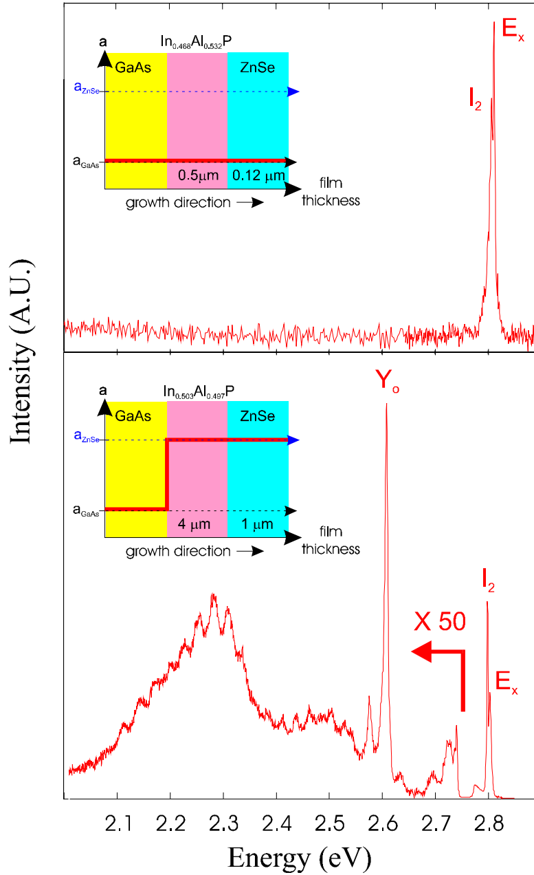
Figure 4-3 (a) 10K PL of pseudomorphic (0.12 μm) ZnSe on In 0.468 Al 0.532 P buffers layer lattice-matched to GaAs (b) 10K PL of 1 μm ZnSe on 4 μm In 0.503 Al 0.497 P buffer layer lattice-matched to ZnSe. The inset in each pane shows the schematics of the lattice constant variation as a function of layer thicknesses.
