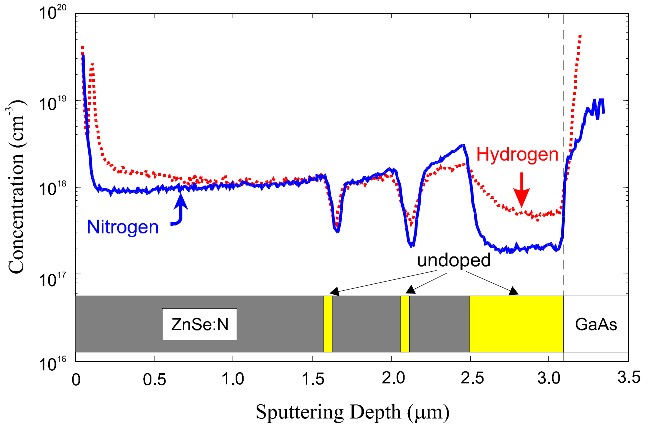
Figure 3–11 SIMS depth profile obtained from a uniformly-doped ZnSe:N epilayer grown by GSMBE on an undoped ZnSe buffer layer. The undoped ZnSe layers, as indicated in the schematic, provide references for the background concentrations of [N] and [H]. The synergistic correlation between [N] and [H] is clearly seen. The dramatic increase in the signal at the surface and at the ZnSe/GaAs interface are due to surface effects and an artifact of the data normalization procedure, respectively.
