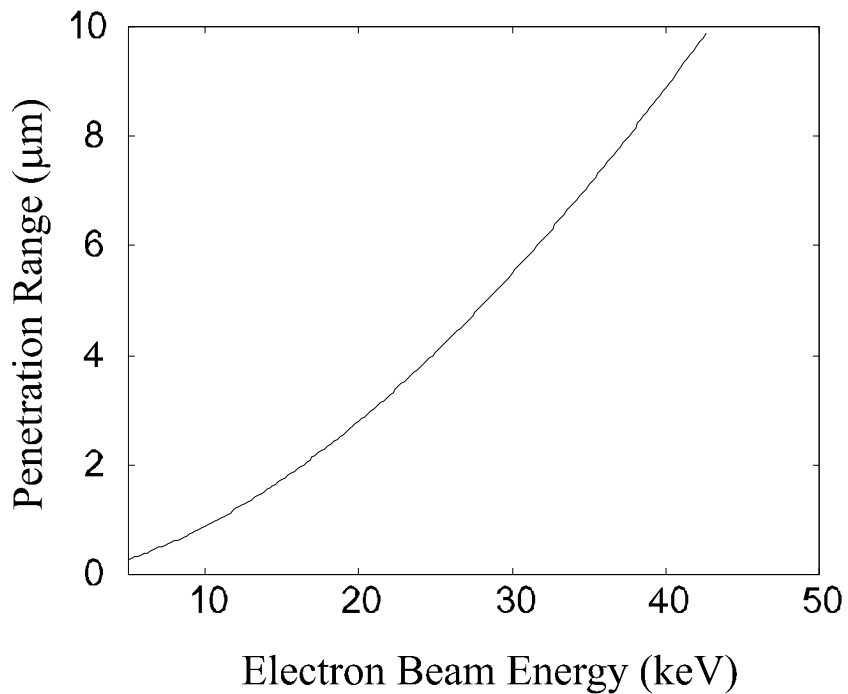
Figure C.3 Calculated electron range as a function of the electron beam energy using equation derived by Kayama et. al. [175].
