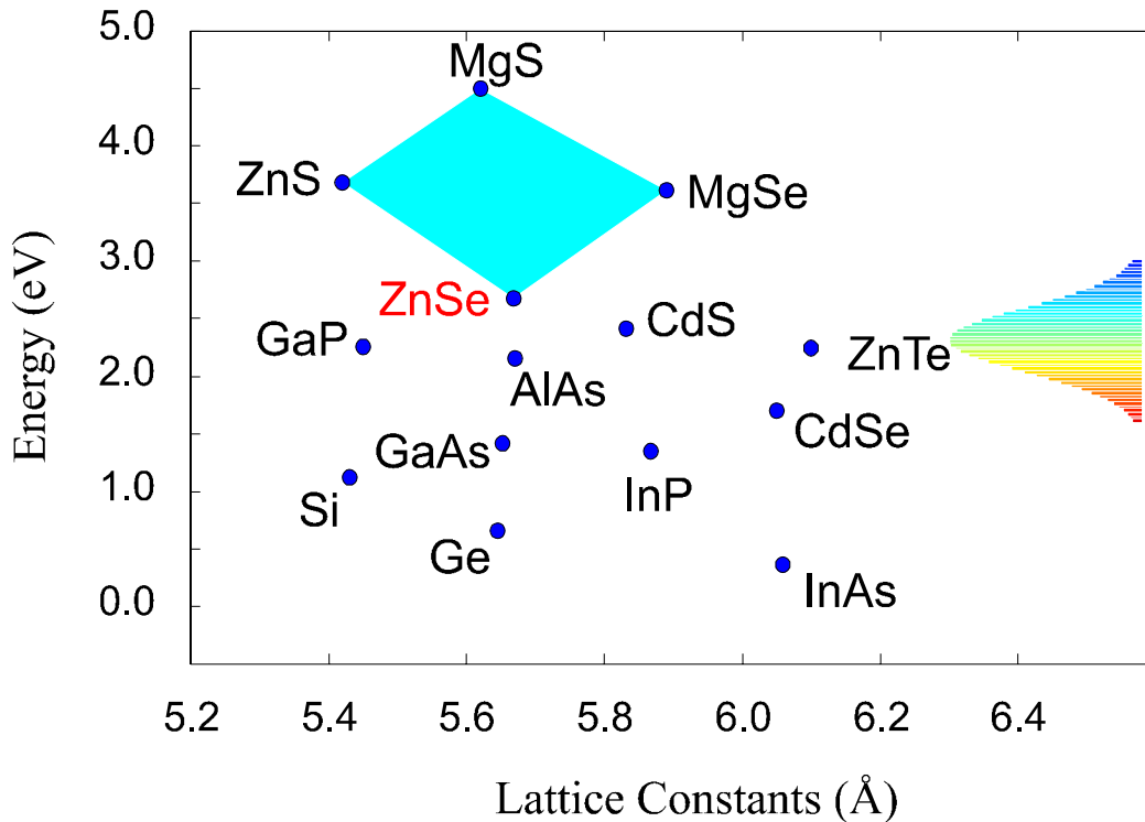
Figure 1–1 Bandgap versus lattice constant diagram for II-VI and III-V binary materials. The curve near the right hand vertical axis schematically indicates human eye's photopic response in the visible region.
