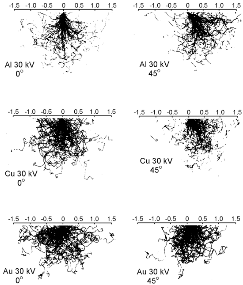
Figure C.2 Calculated electron trajectories for a 30kV beam in Al, Cu, and Au for both 0^\circ (normal) and 45^\circ incidences as indicated. Note that the horizontal axis is given in units of \rho \cdot x ( \text{mg}/\text{cm}^2 ). Figure adapted from [174]
