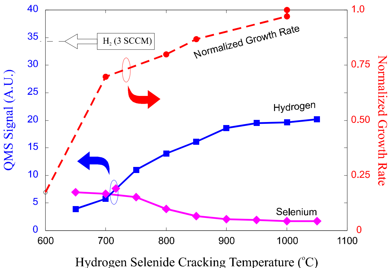
Figure 3–14 Comparison of the H 2 and elemental selenium signals (left vertical axis) as seen by a QMS that is generated as a by-product of the H 2 Se cracking; also shown is the signal obtained by 3 SCCM of intentionally introduced H 2 gas. The right vertical axis depicts the relative growth rates (normalized to neutralize the effect of varying group II fluxes) as a function of the H 2 Se cracker cell.
