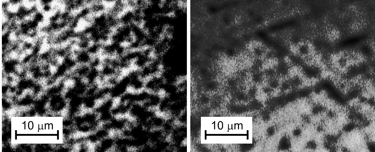
(a) Graded InGaAlP ( a=a_{\text{ZnSe}} )
