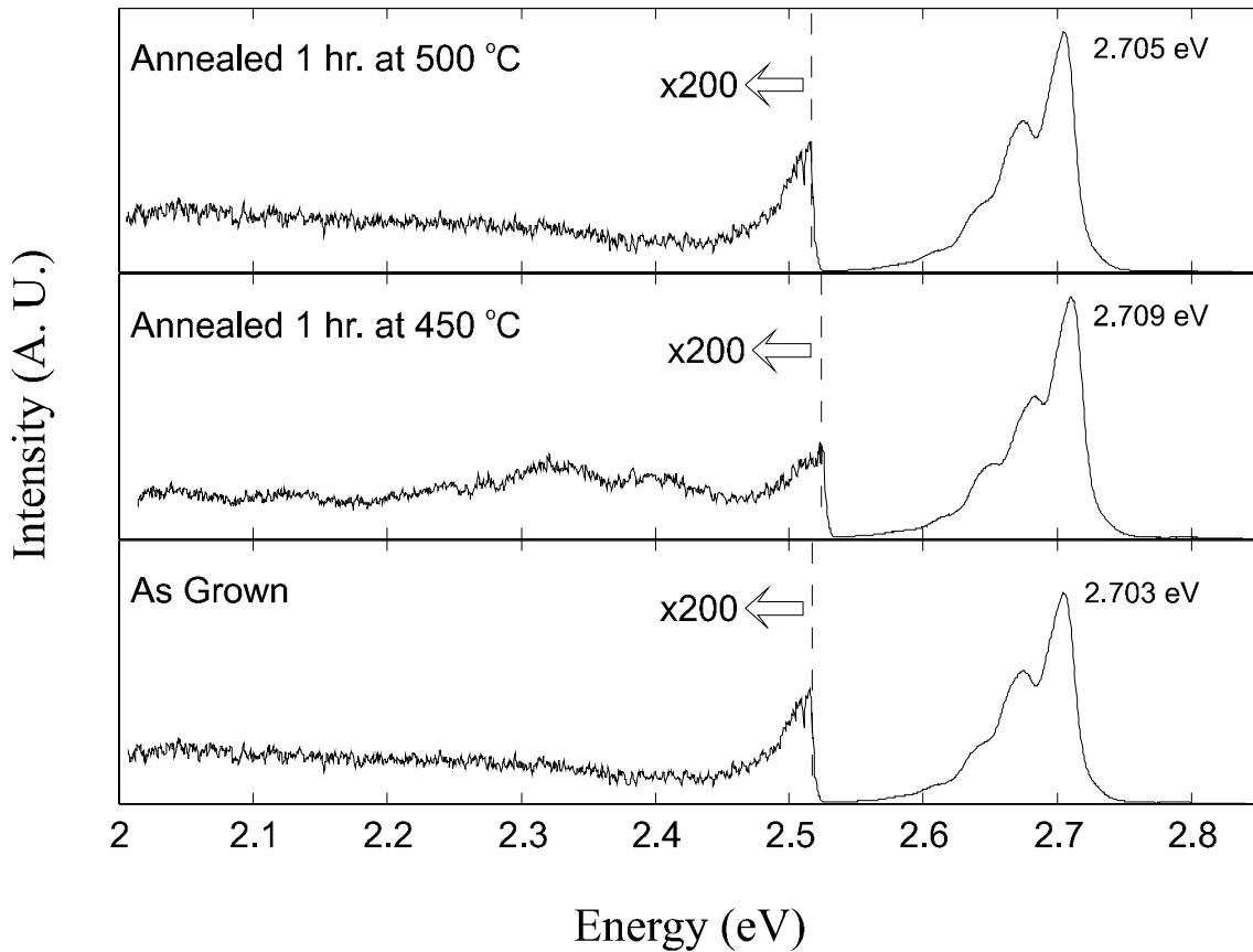
Figure 3–17 The effect of long term annealing on the photoluminescent properties of ZnSe:N grown by GSMBE under different annealing temperatures.
