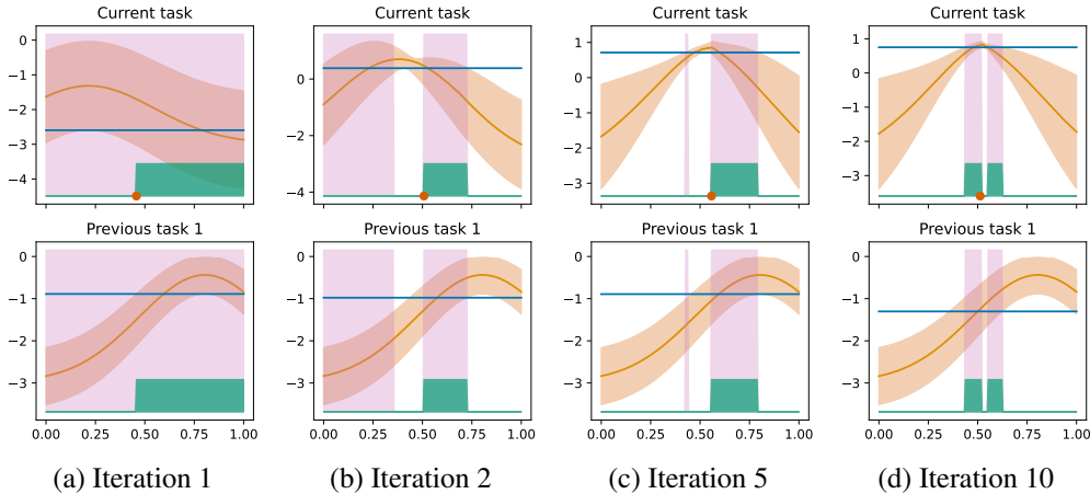
Figure 5: Visualization of the query set \mathcal{Q}_t and the probable local maximizer sets \mathcal{P}_{\tau|\mathcal{Q}_t} when the prior task has poorly-estimated VaR. The figures in each column share the same x -axis. The top figure displays the GP posterior mean (the orange line) along with the lower and upper bounds (the orange shaded area) for the blackbox function of the current task. The bottom figure displays the same information for the prior tasks. The blue line in both figures indicates the maximum lower bounds, while the pink shaded area represents the V-set \mathcal{Q}_t . Although \mathcal{Q}_t is defined based on the bounds of the blackbox function of the current task, it is also visualized in the bottom figures to aid in visualizing the probable local maximizer set \mathcal{P}_{\tau|\mathcal{Q}_t} . The green shaded areas in the bottom figures illustrate the probable local maximizer set \mathcal{P}_{\tau|\mathcal{Q}_t} for the prior task. In the top figures, the green shaded areas indicate the count of probable local maximizer sets to which an input belongs (a higher green area corresponds to a larger number of probable local maximizer sets). The red dot shows the input query \mathbf{x}_t .
