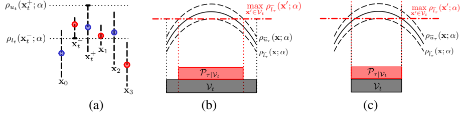
Figure 1: (a) Plot of \mathcal{V}_t = \{\mathbf{x}_0, \mathbf{x}_t^+, \mathbf{x}_2\} with \lambda = 0 and \eta = 1 . The dashed line shows the confidence interval of \rho_f(\mathbf{x}_*; \alpha) . While \mathbf{x}_t^- and \mathbf{x}_1 violate UC, \mathbf{x}_3 violates OC. (b) Plot of an informative prior task \tau where \mathcal{V}_t \setminus \mathcal{P}_{\tau|\mathcal{V}_t} \neq \emptyset . (c) Plot of an uninformative prior task \tau where \mathcal{P}_{\tau|\mathcal{V}_t} = \mathcal{V}_t .
