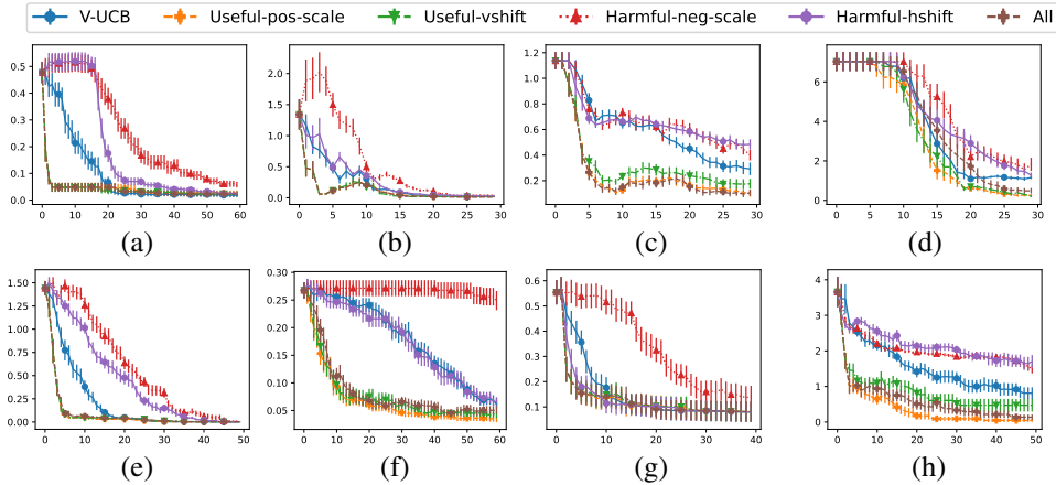
Figure 2: Plots of the regret at the recommended input against the BO iteration in experiments with (a) a Gaussian curve, (b) the Branin-Hoo function, (c) the Goldstein-Price function, (d) the six-hump camel function, (e) the Hartmann-3D function, (f) the Hartmann-6D function, (g) the yacht hydrodynamics dataset, and (h) the portfolio optimization dataset.
